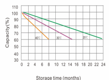
Self-discharge characteristic
