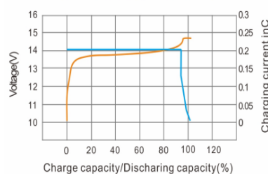
0.2C CC-CV charge chararveristic
