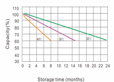
Self-discharge characteristic
